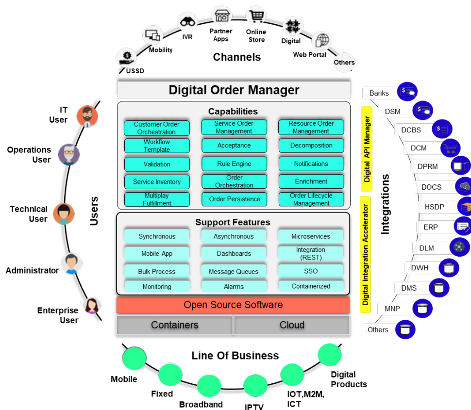
Figure 5 DOM Scope
